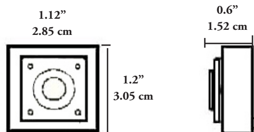
CVC6130K - PINHOLE LENS
